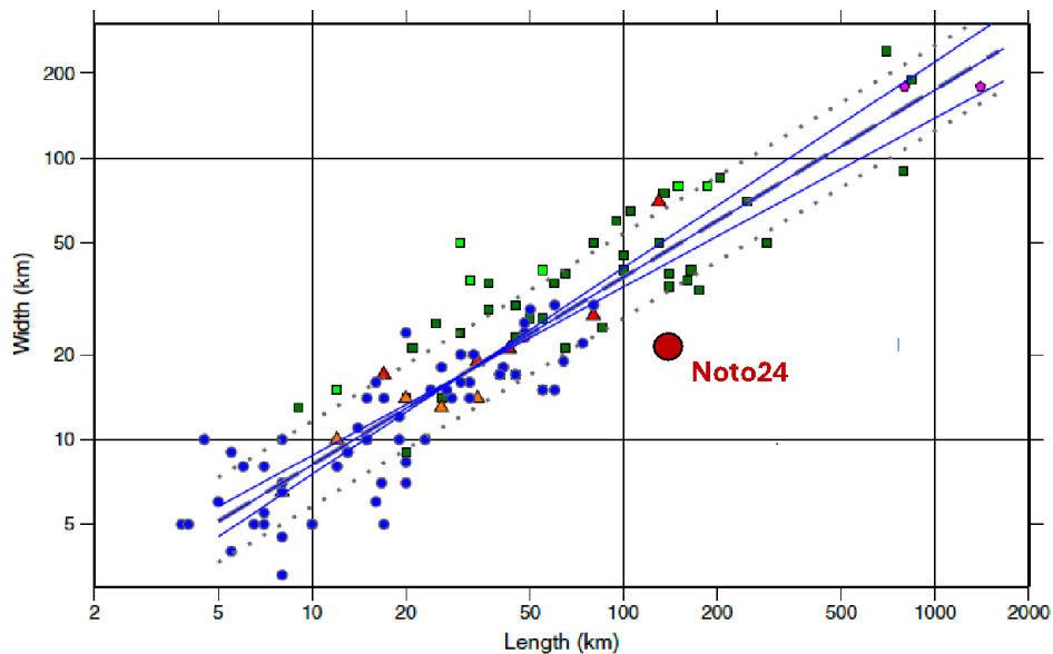
Figure 3.20. Width versus length for normal and reverse dip-slip interplate faults compiled by Leonard (2010); lines are from his scaling analysis. The least-squares estimate (dashed line) has a slope of 0.668. Points with different symbols and colors are from different published catalogs (see Leonard, 2010, fig. 1 for key). The Noto24 rupture (large red dot) has a very high aspect ratio (~7), which has been attributed to the energetic rupturing of multiple strong asperities. [Source: Leonard (2010), fig. 1.]
