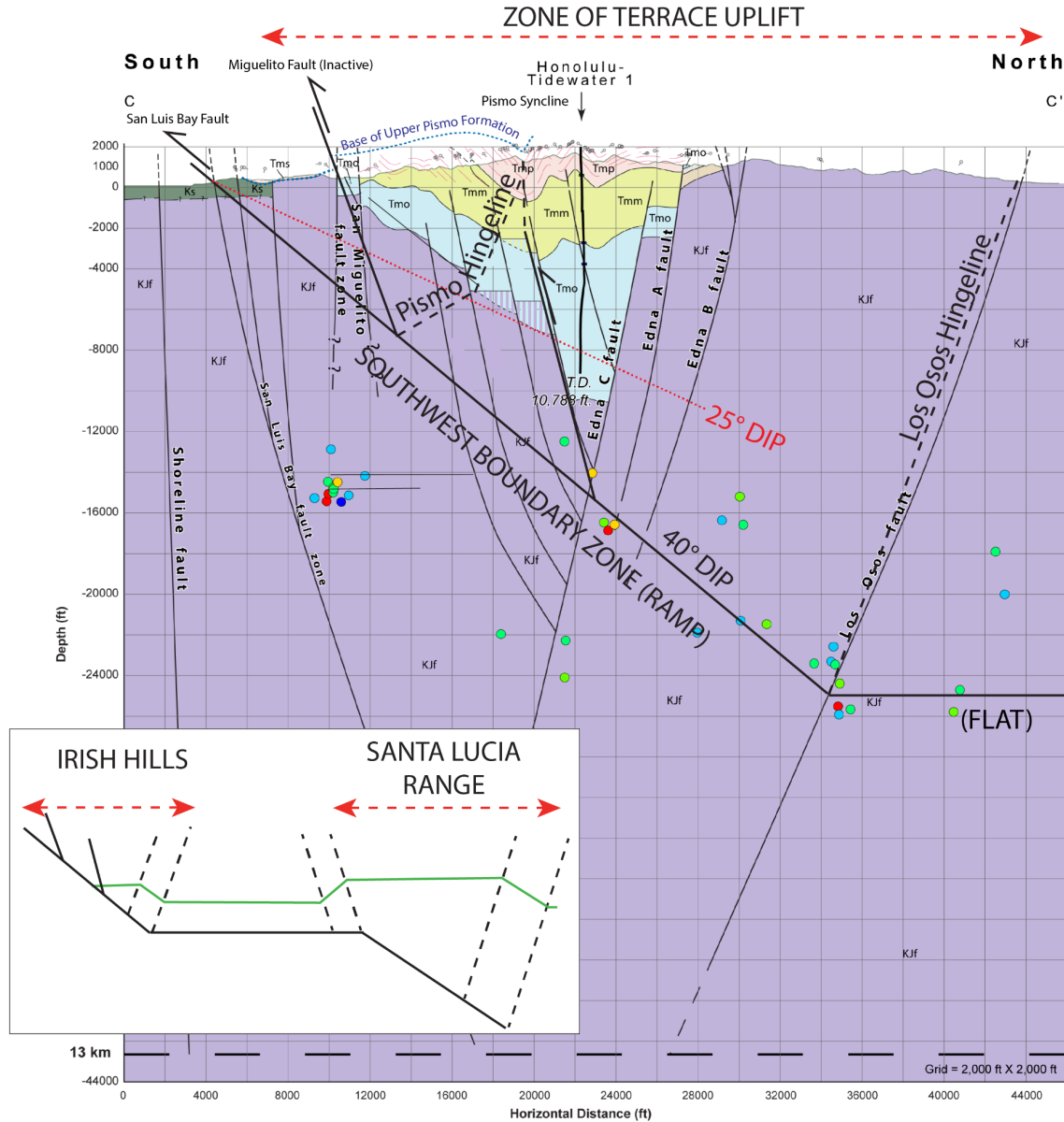
Figure 3.5. Cross-section C-C' from PG&E (2014), annotated with fault-bend fold model for the SWBZ. Tilting of the south limb of Pismo Syncline occurred due to slip transfer from SWBZ ramp to the Miguelito fault, an inverted normal fault that formed the southern margin of the Pismo basin. Hingeline of the Pismo Syncline refracts upwards to accommodate bedding-parallel shear of layered sedimentary rocks overlying Franciscan basement. Note patterned areas showing revised layer positions beneath syncline axis. Base of Upper Pismo Formation in the hangingwall of the Miguelito fault projected into section from east. Red dotted line depicts a hypothetical San Luis Bay fault with 25° dip (compare to Figure 2.3). This fault configuration would intersect the Obispo formation and the Tidewater-Honolulu oil well. Diagram at lower left shows a ramp-flat-ramp model that extends the SWBZ northward to root beneath the southern Santa Lucia range. Zones of marine-terrace uplift correspond to fault ramps.
