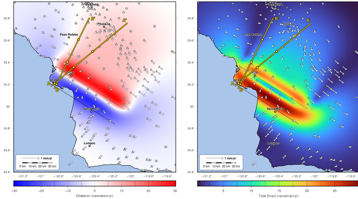
Figure B.6. (a) Dilatational and (b) total strain rates from a 3D kinematic dislocation model utilizing a 15 km locking depth and a 40° dipping fault with 2.5 mm/yr of slip similar to the geometry of shallowest dipping fault in the SSC24 (SSC24 incorporates a minimum dip of 45°). Plotting conventions are the same as in Figure 3.16.
